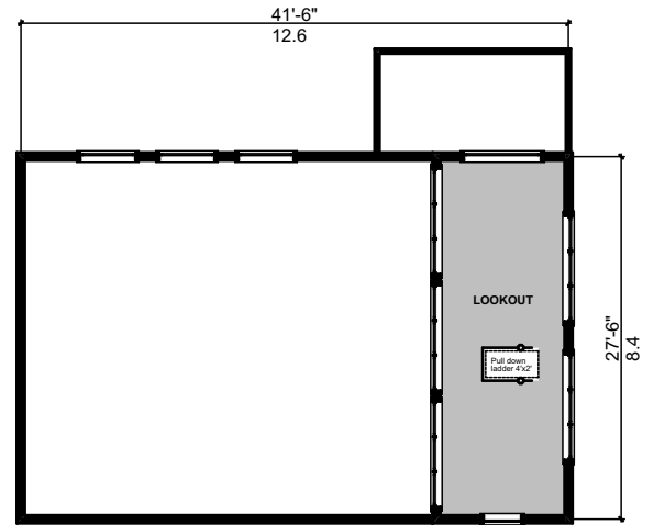
SECOND FLOOR PLAN AREA: 294 SQ. FT. / 27.3 SQ. M
