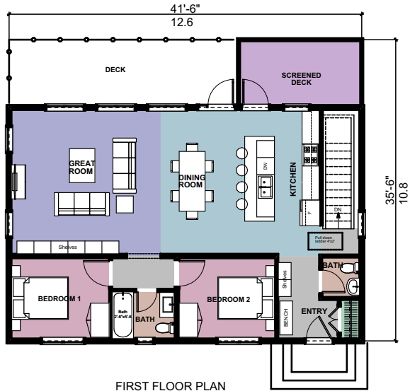
FIRST FLOOR PLAN AREA: 1176 SQ.FT. / 109.3 SQ.M
