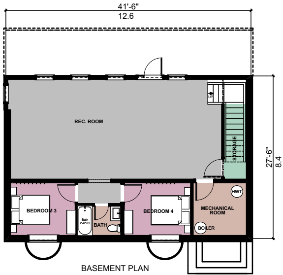
BASEMENT PLAN AREA: 1176 SQ. FT. / 109.3 SQ.M
